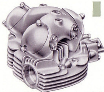
TWIN HEAD. A clean light alloy head offering large cooling area and providing efficient inlet and exhaust ports. The O.H.V. rockers are carried integrally.
