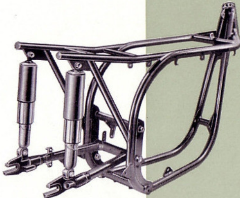
FRAME. The really outstanding handling of this frame must be experienced to be believed. This is now used on all models from 350 c.c. upwards.
