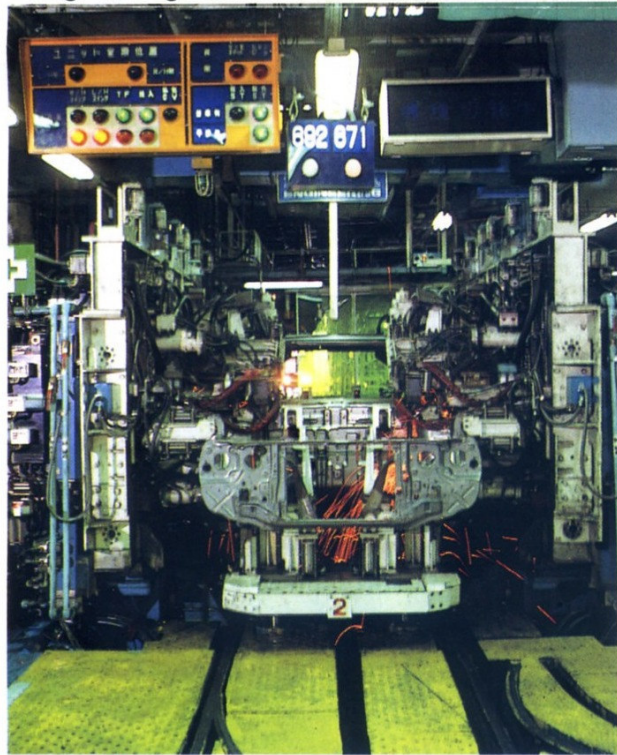
▼ Welding Machine made by Honda Engineering Co., Ltd.
