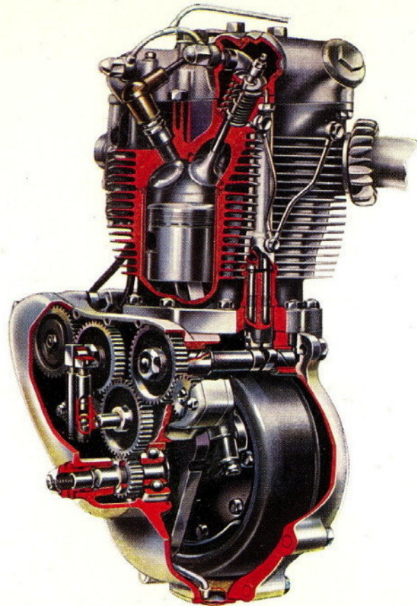
The Triumph-pioneered vertical twin cylinder o.h.v. engine, famed for its power output, economy and complete reliability.
