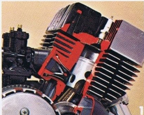
1. Twin powerhouse with TORQUE INDUCTION ® means 7-port power that gives Yamaha more horsepower at all rpm's.
