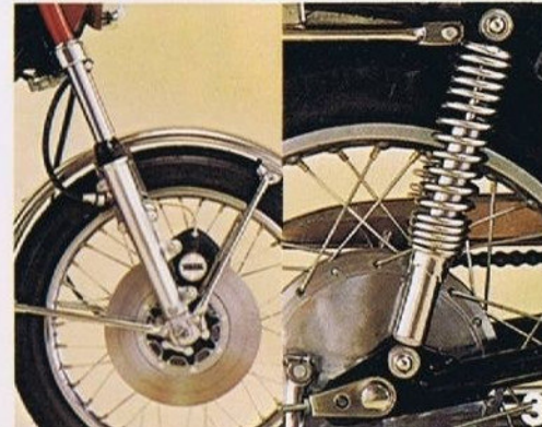
3. Enduro type front forks are acknowledged as one of the world's best designs. Outstanding comfort and safety, especially when coupled with fade-free front disc brake. Adjustable rear shocks with 3 positions for the perfect ride.
